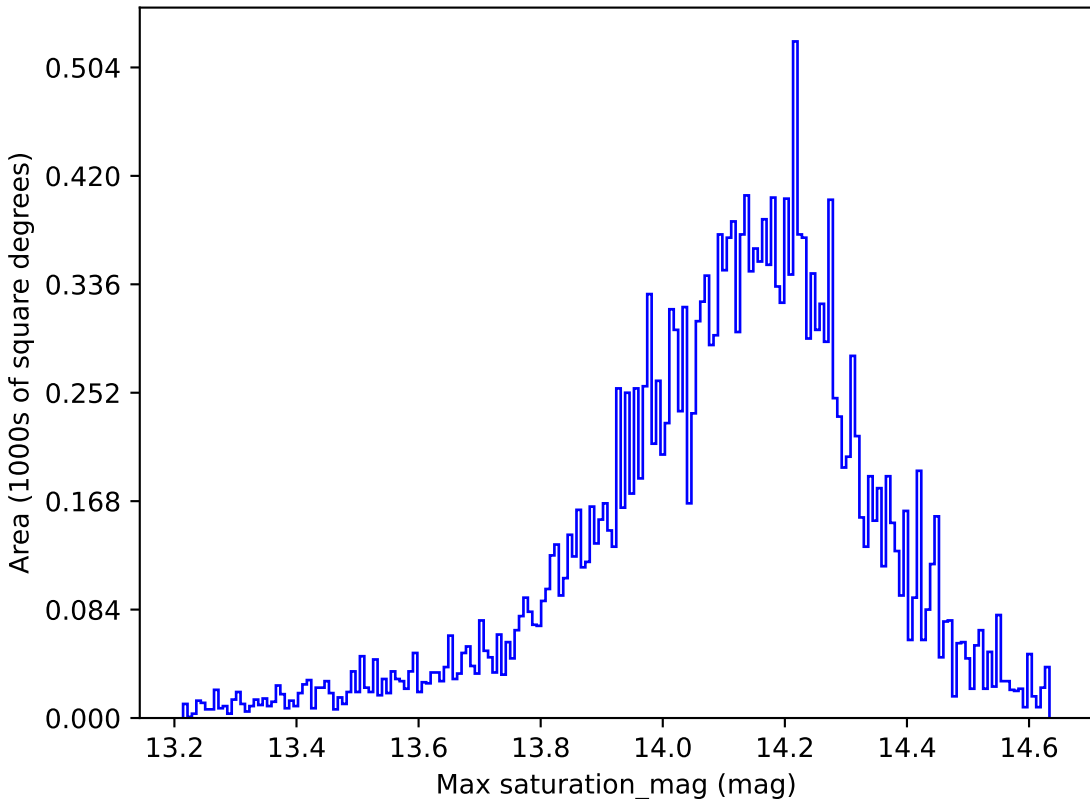
too_10_4v3.4_10yrs All sky y band: Max saturation_mag
