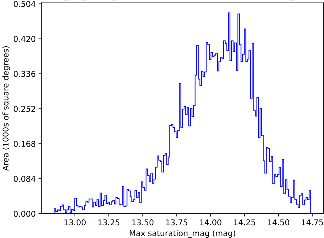
too_10_4v3.4_10yrs All sky u band: Max saturation_mag
