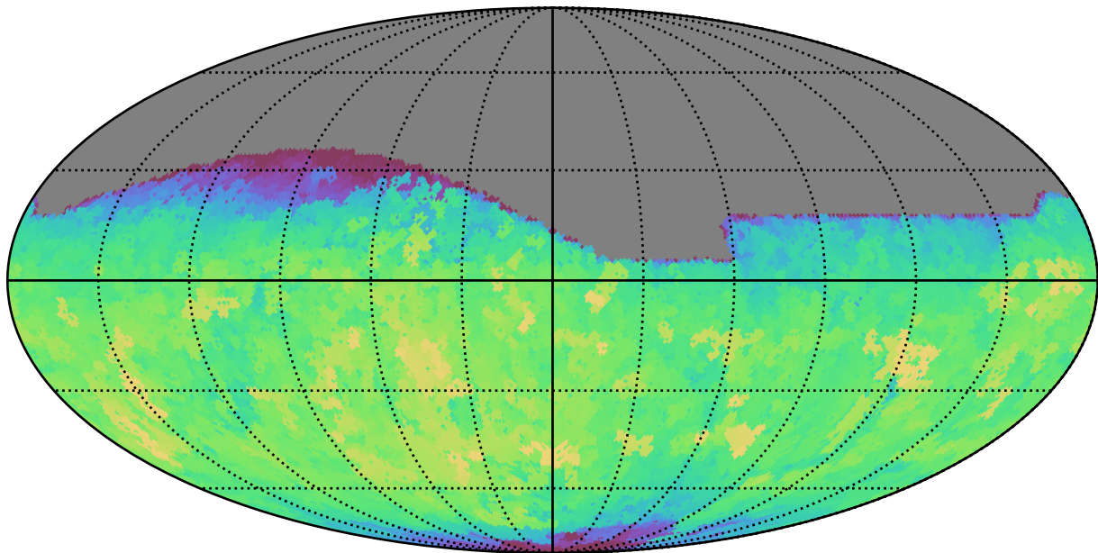
too_10_4v3.4_10yrs All sky r band: Max saturation_mag
