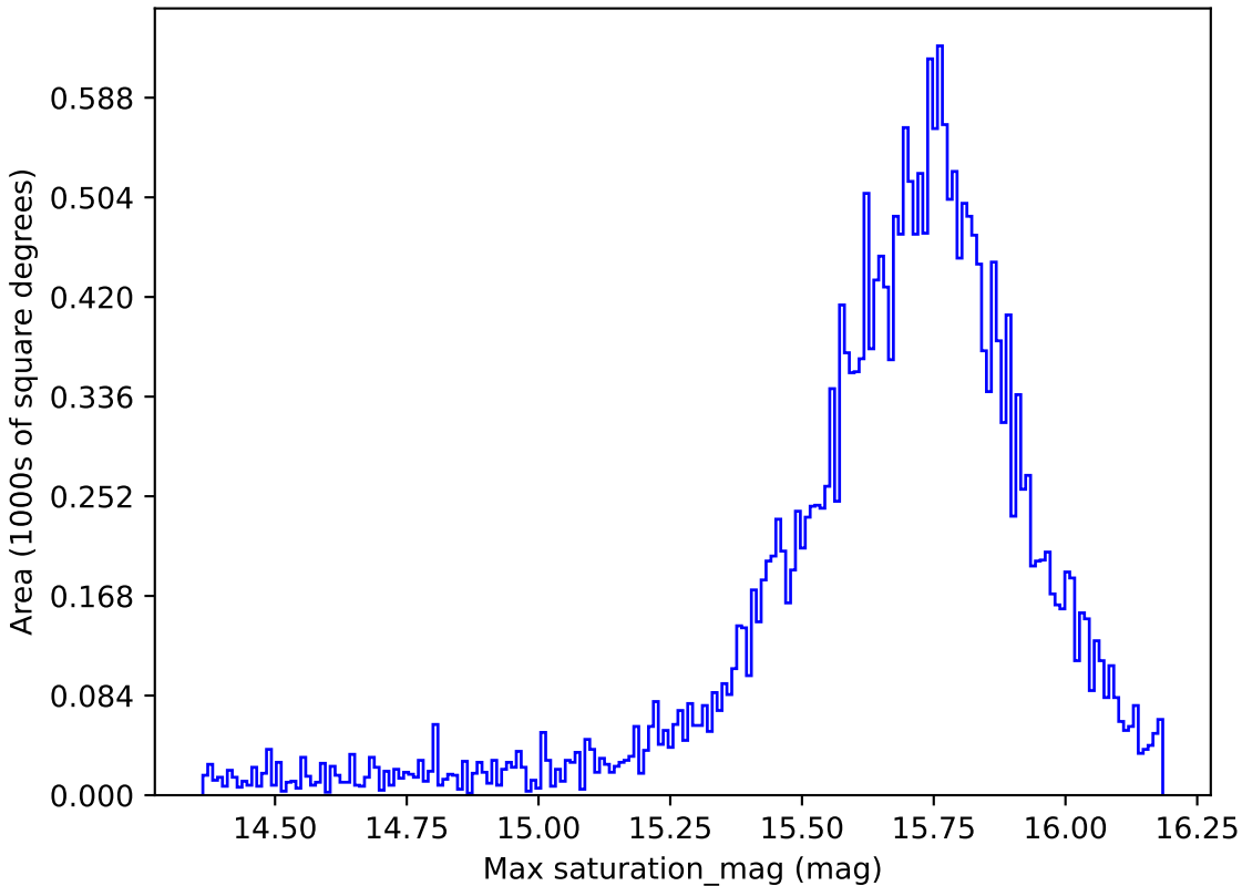
too_10_4v3.4_10yrs All sky r band: Max saturation_mag
