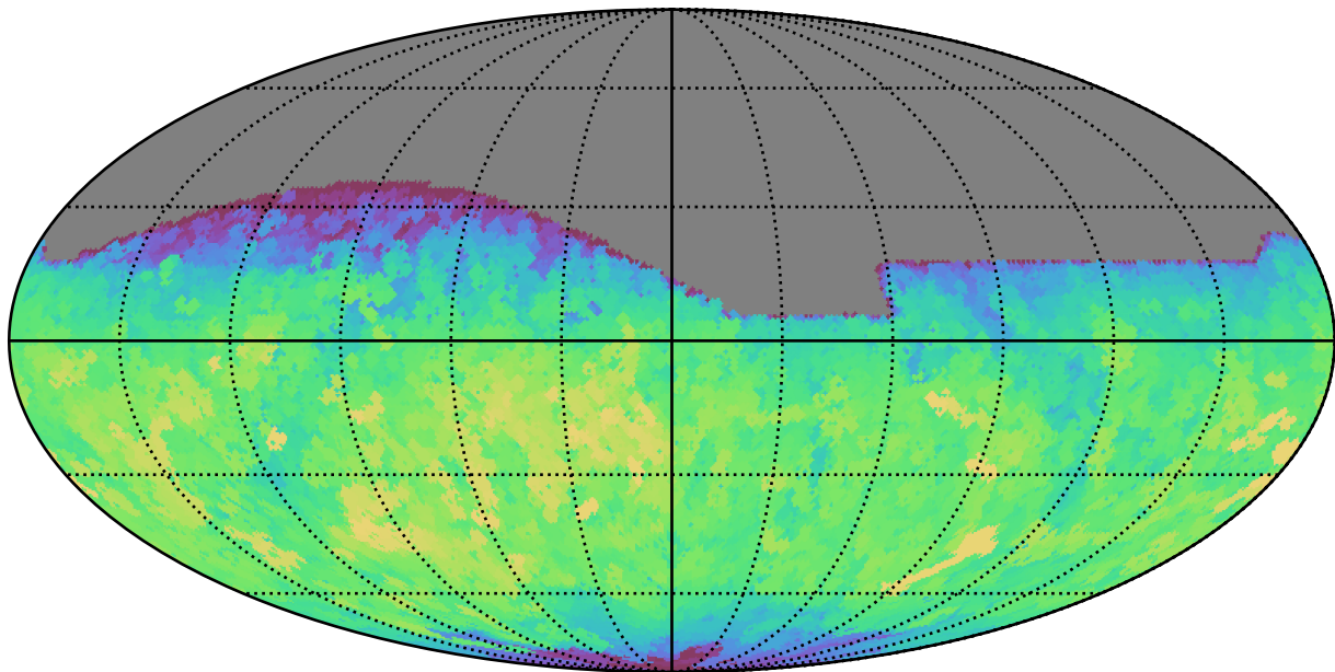
too_10_4v3.4_10yrs All sky i band: Max saturation_mag
