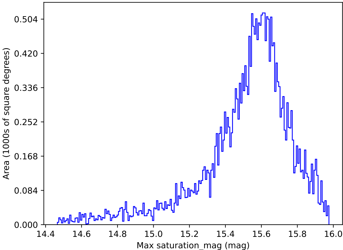
too_10_4v3.4_10yrs All sky i band: Max saturation_mag
