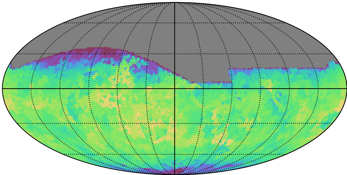
too_10_4v3.4_10yrs All sky g band: Max saturation_mag
