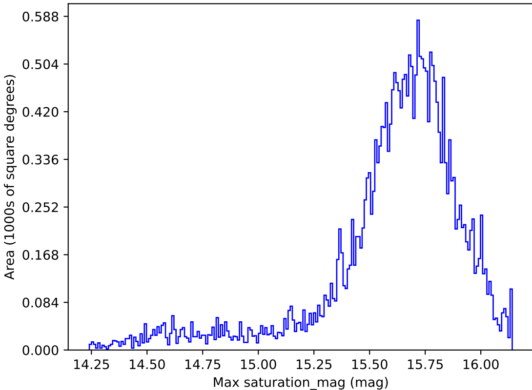
too_10_4v3.4_10yrs All sky g band: Max saturation_mag
