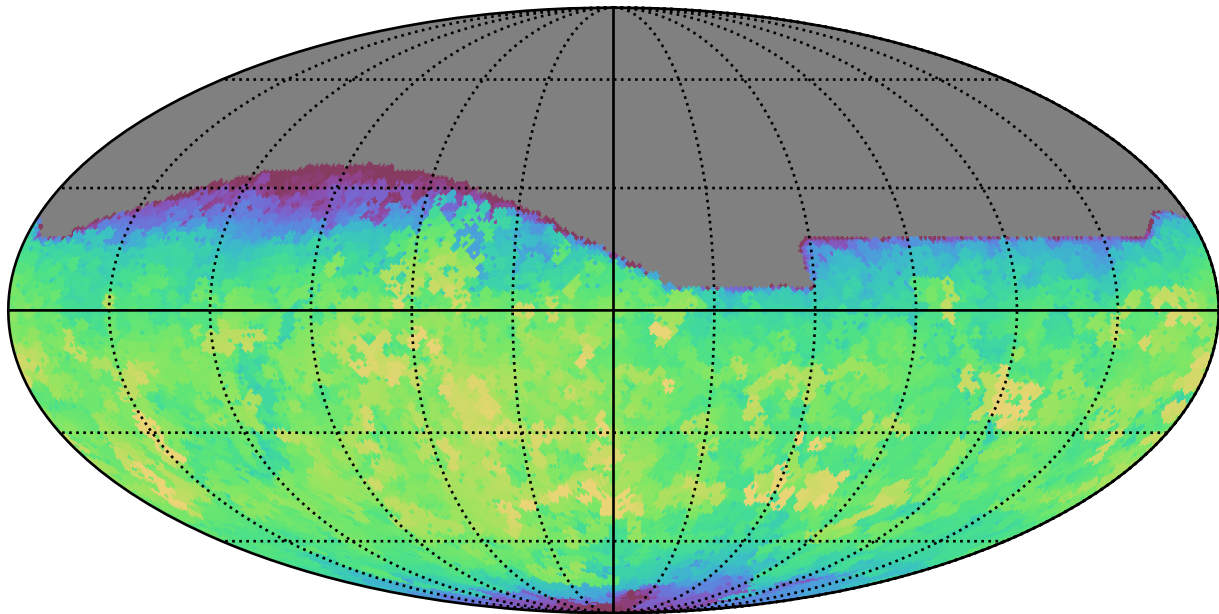
too_10_4v3.4_10yrs All sky all bands: Max saturation_mag
