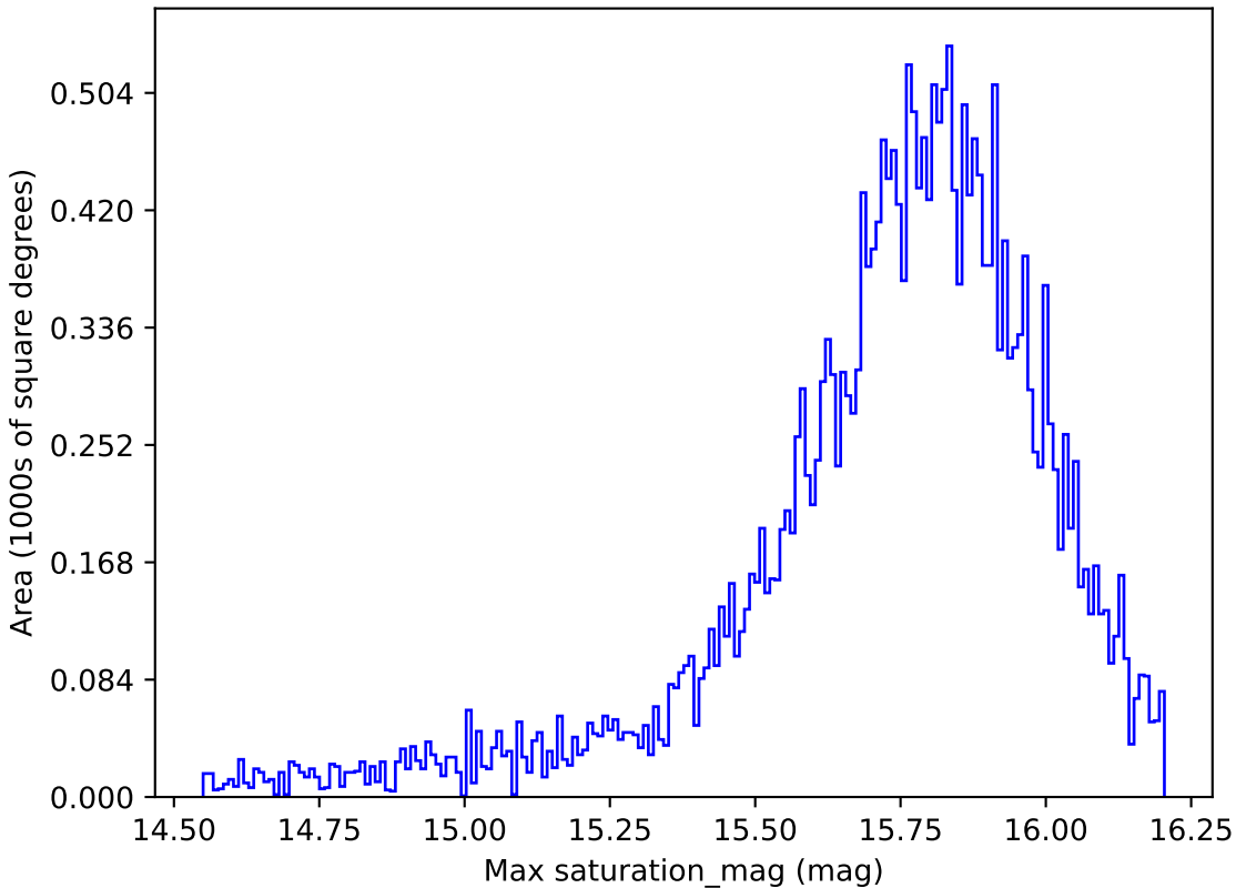
too_10_4v3.4_10yrs All sky all bands: Max saturation_mag
