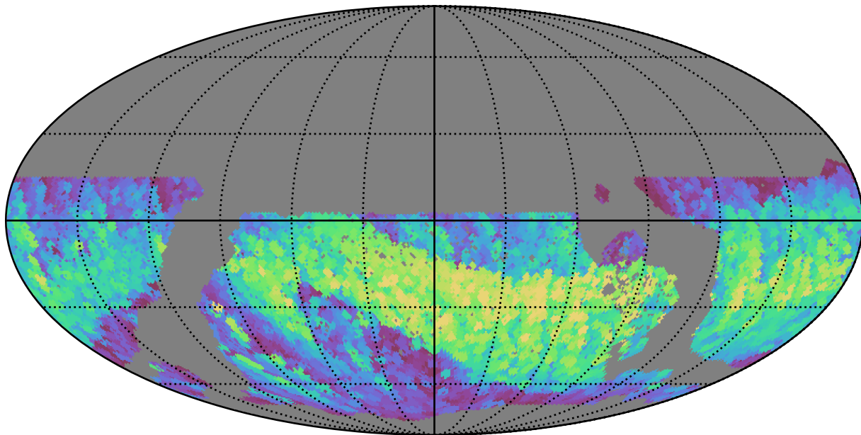
too_10_4v3.4_10yrs WFD z band: Max normairmass
