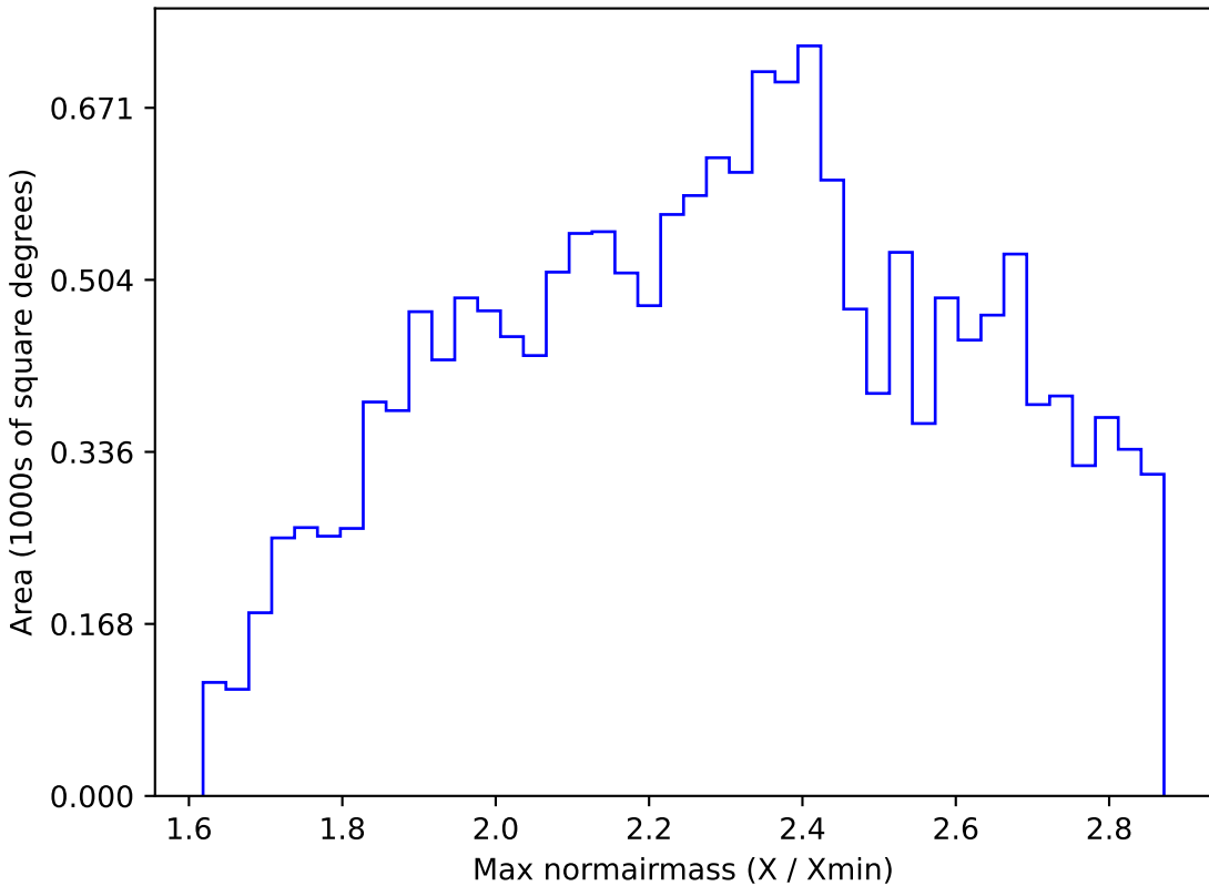
too_10_4v3.4_10yrs WFD z band: Max normairmass
