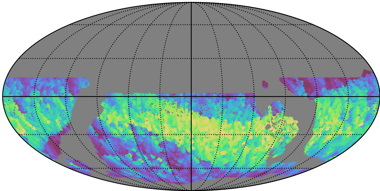
too_10_4v3.4_10yrs WFD i band: Max normairmass
