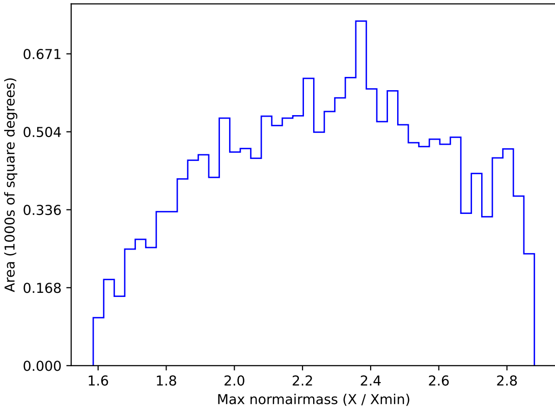
too_10_4v3.4_10yrs WFD i band: Max normairmass
