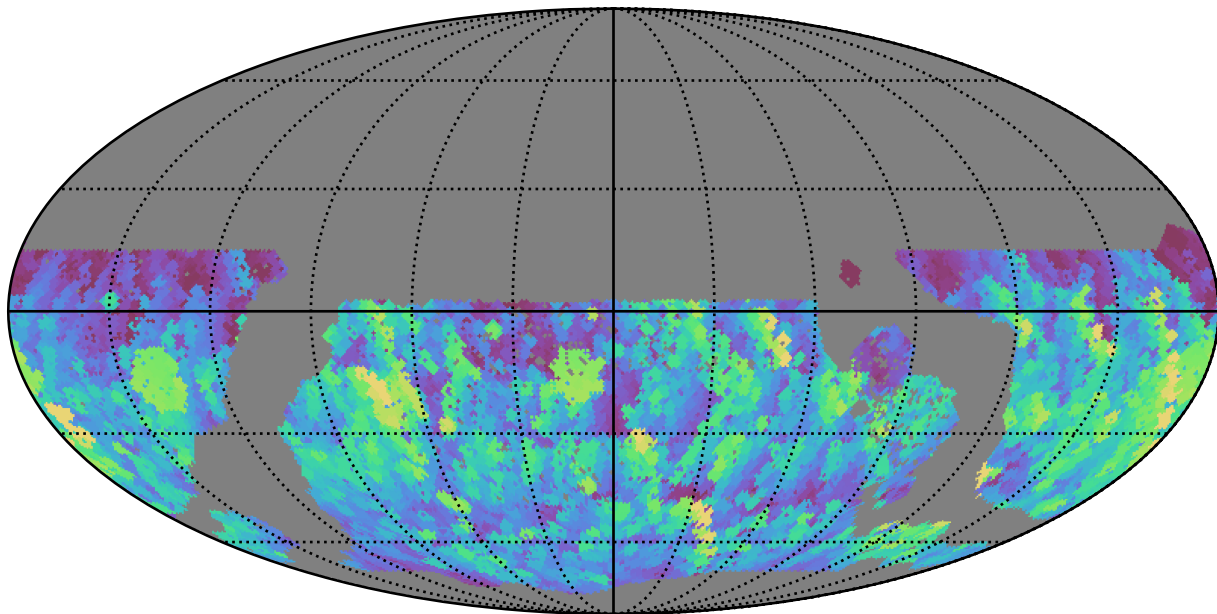
too_10_4v3.4_10yrs WFD g band: Max normairmass
