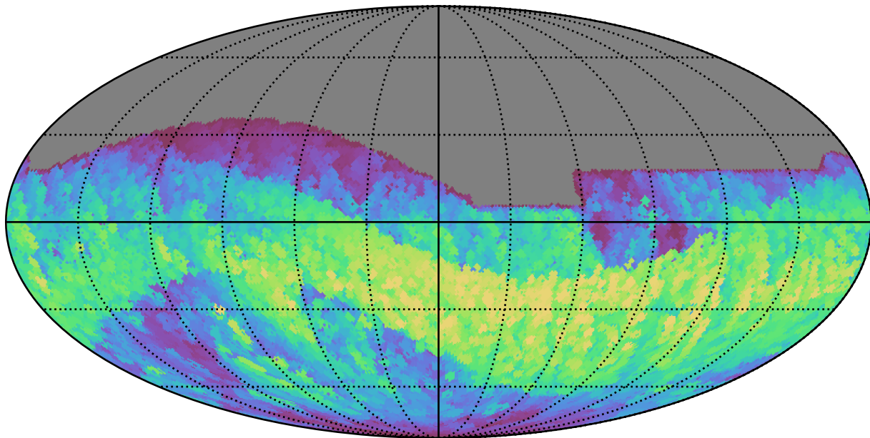
too_10_4v3.4_10yrs All sky z band: Max normairmass
