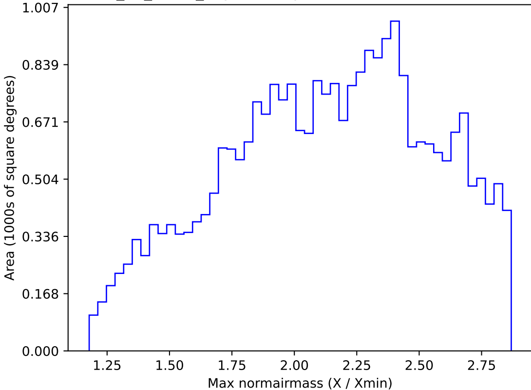
too_10_4v3.4_10yrs All sky z band: Max normairmass
