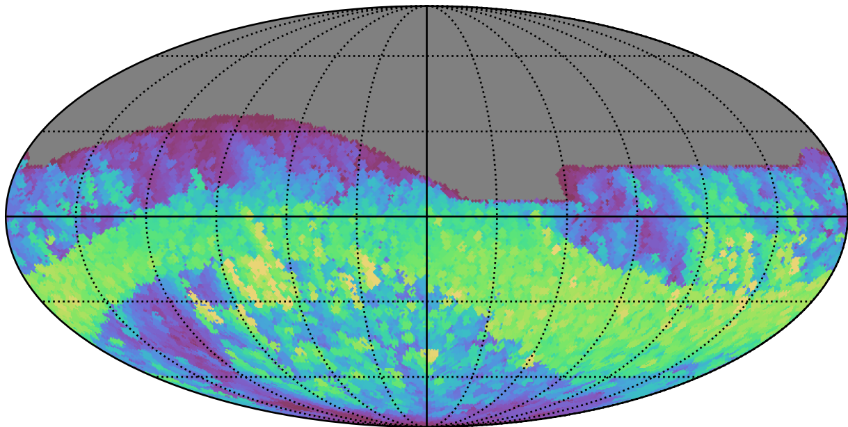
too_10_4v3.4_10yrs All sky r band: Max normairmass
