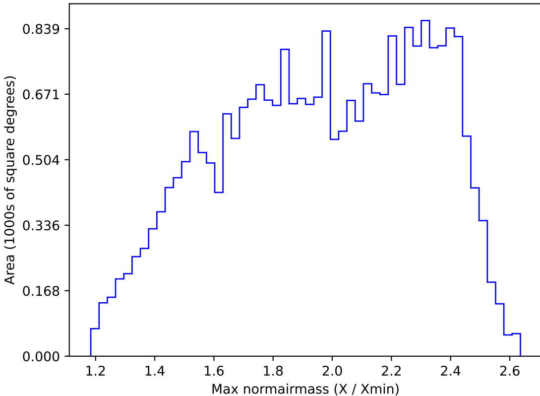
too_10_4v3.4_10yrs All sky r band: Max normairmass
