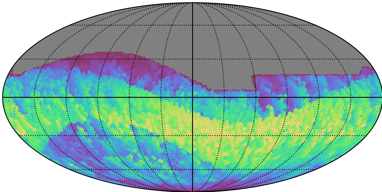
too_10_4v3.4_10yrs All sky i band: Max normairmass
