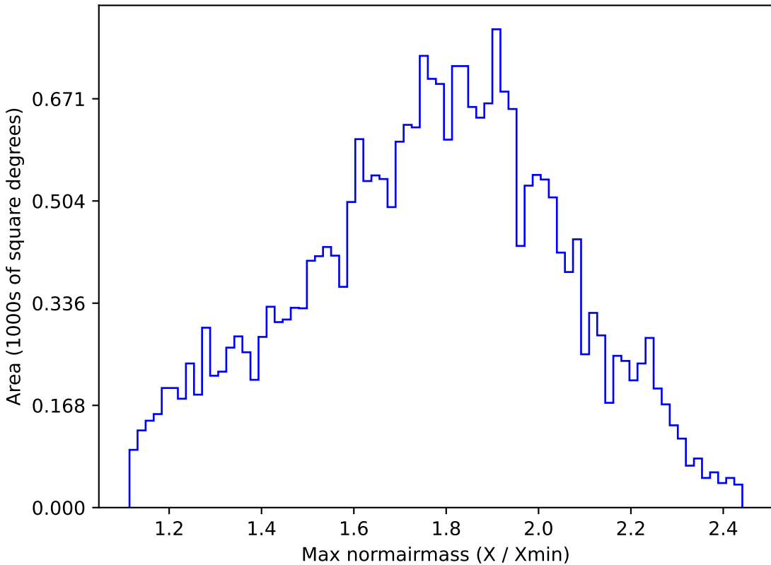
too_10_4v3.4_10yrs All sky g band: Max normairmass
