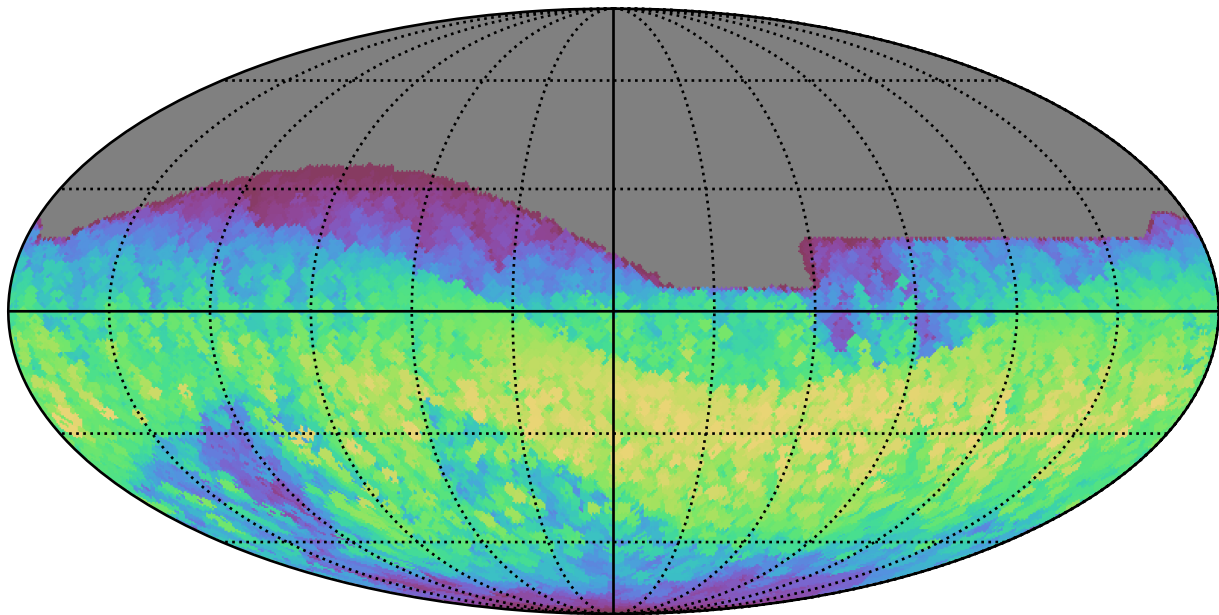
too_10_4v3.4_10yrs All sky all bands: Max normairmass
