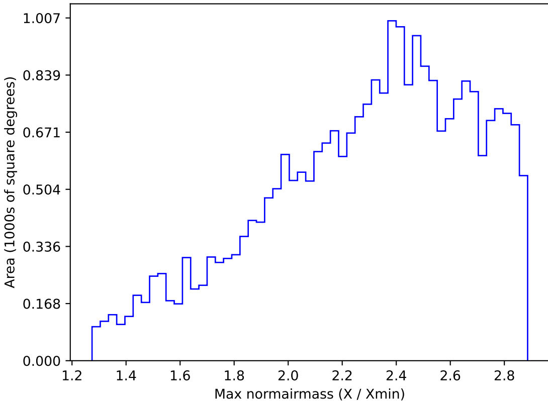
too_10_4v3.4_10yrs All sky all bands: Max normairmass
