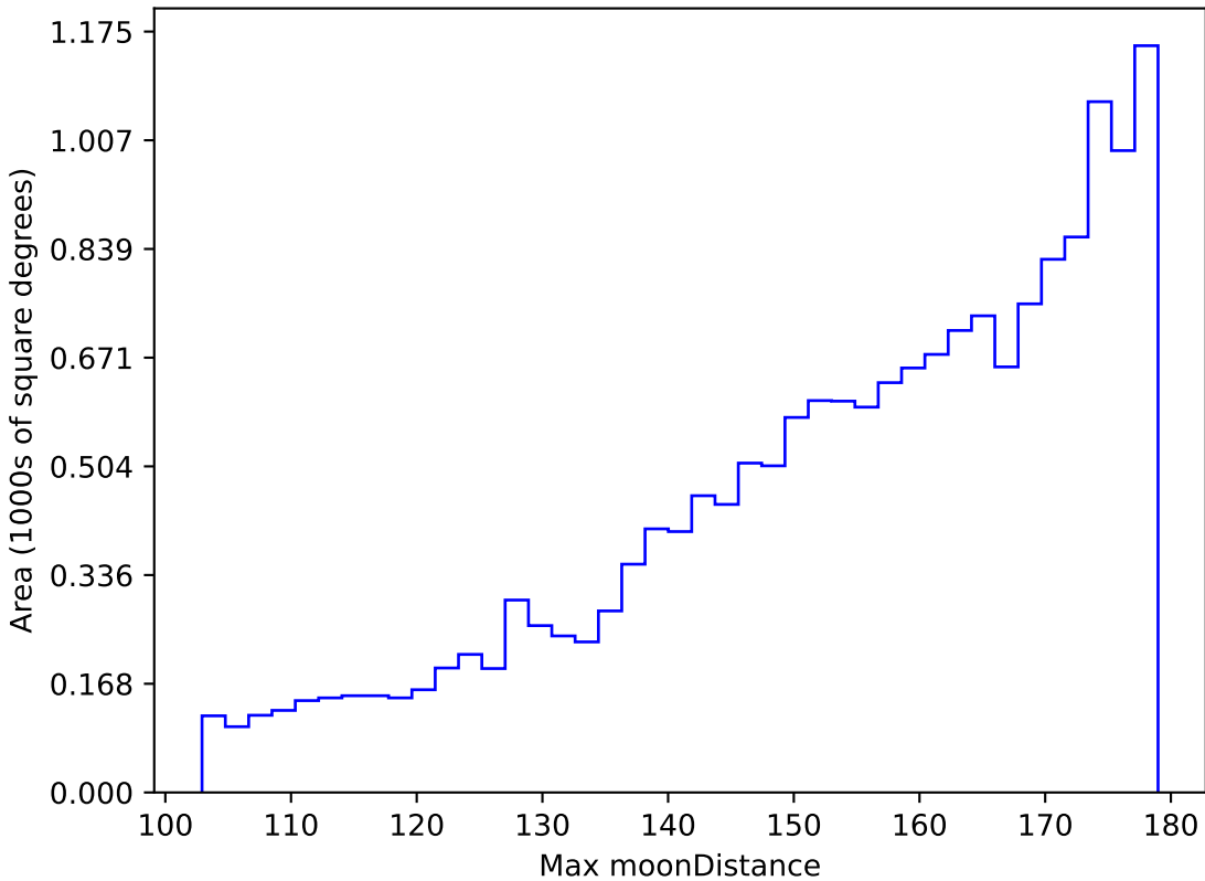
too_10_4v3.4_10yrs WFD z band: Max moonDistance
