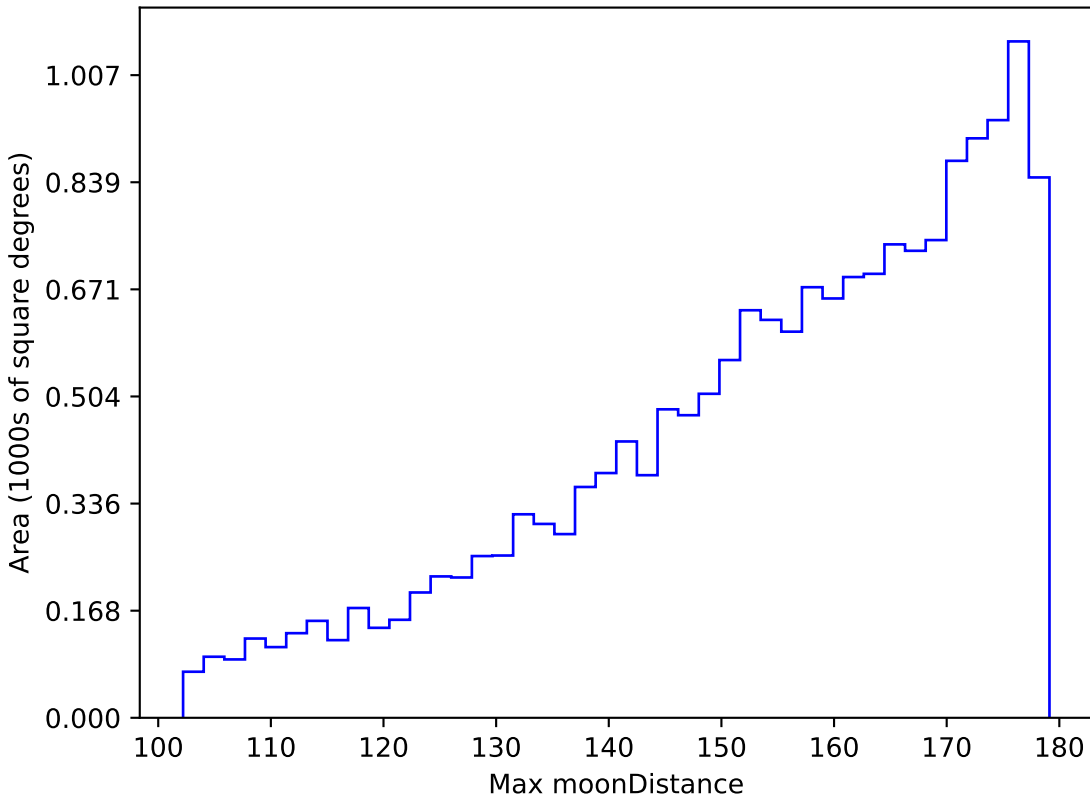
too_10_4v3.4_10yrs WFD u band: Max moonDistance
