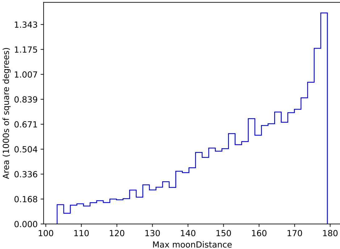
too_10_4v3.4_10yrs WFD i band: Max moonDistance
