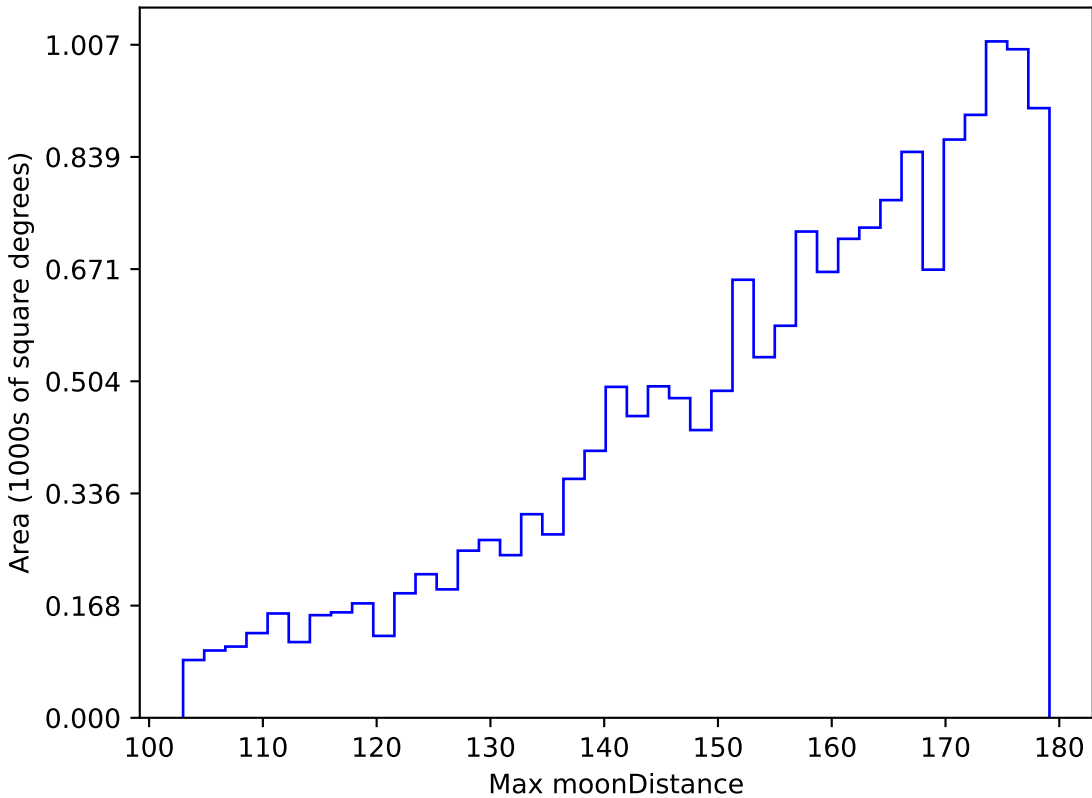
too_10_4v3.4_10yrs WFD g band: Max moonDistance
