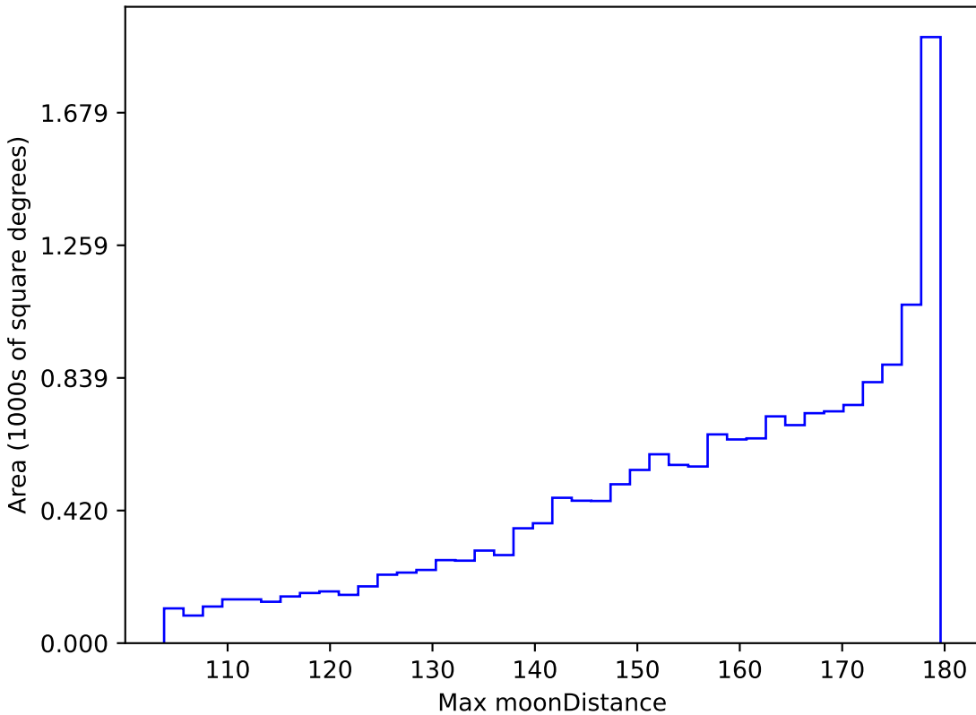
too_10_4v3.4_10yrs WFD all bands: Max moonDistance
