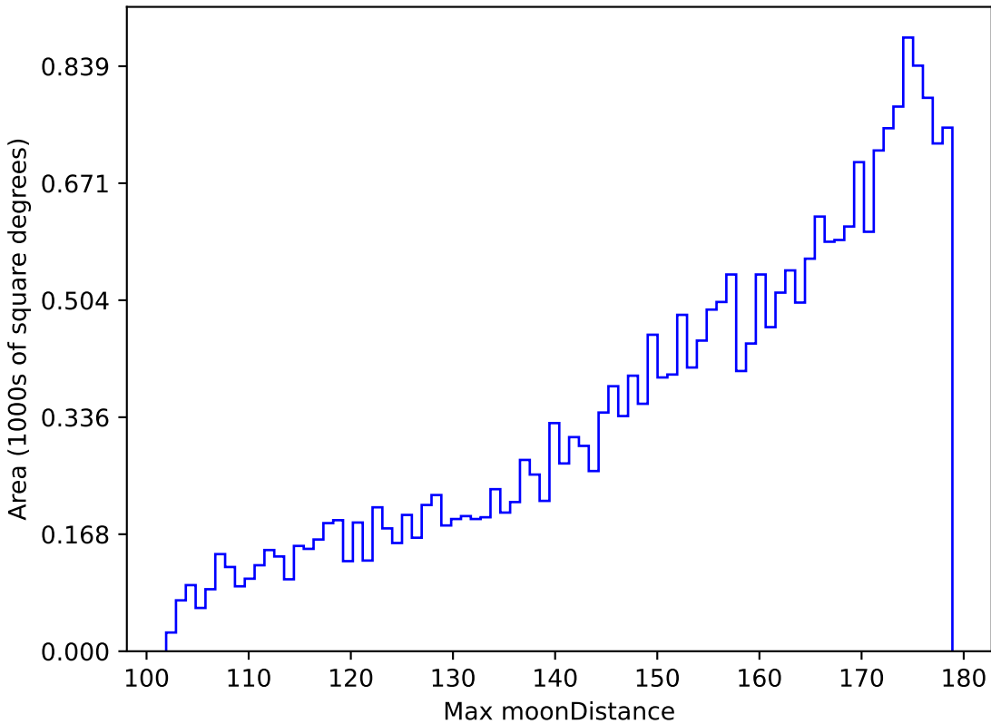
too_10_4v3.4_10yrs All sky z band: Max moonDistance
