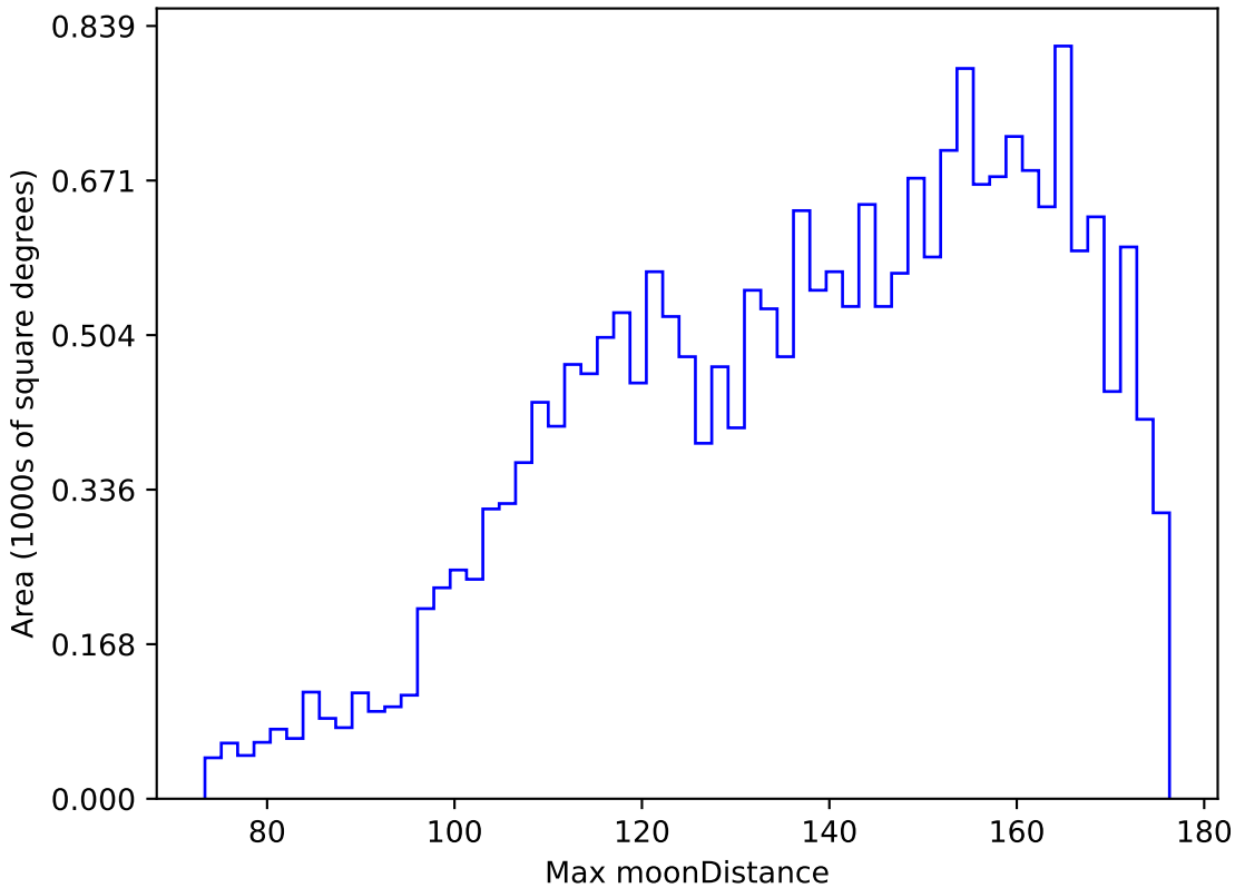
too_10_4v3.4_10yrs All sky y band: Max moonDistance
