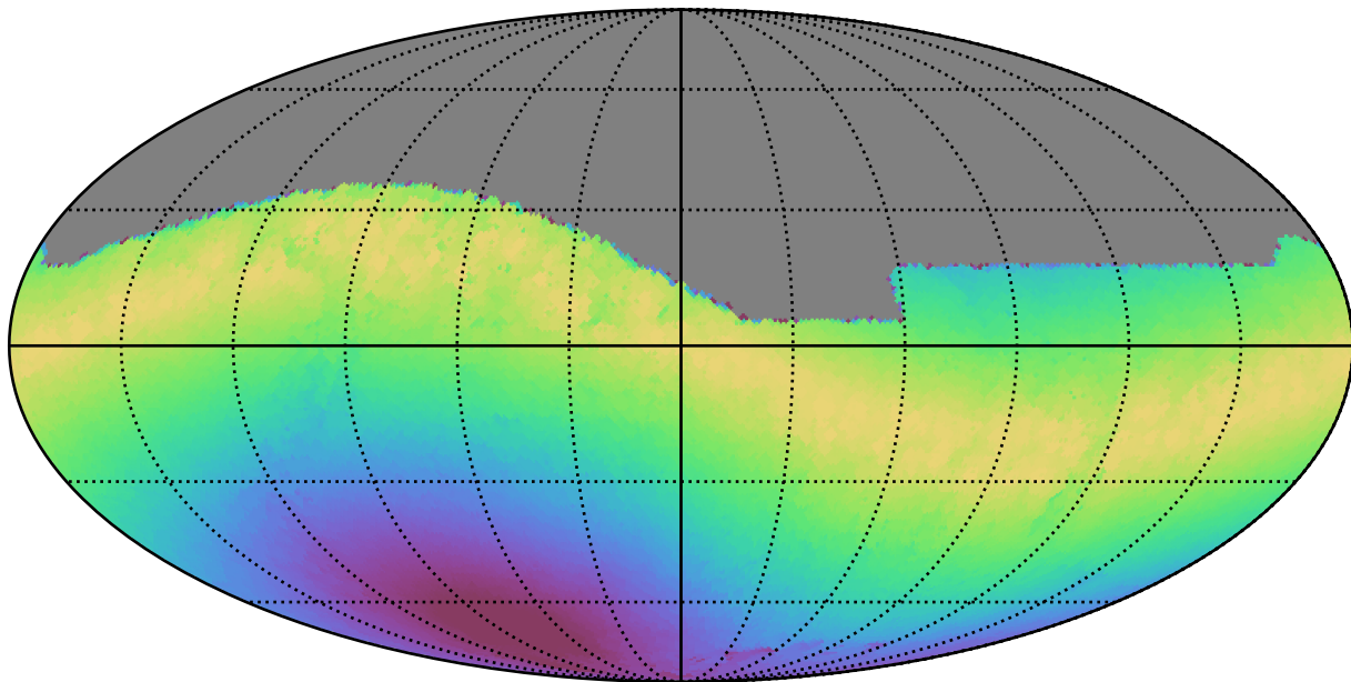
too_10_4v3.4_10yrs All sky r band: Max moonDistance
