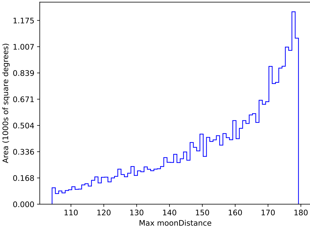
too_10_4v3.4_10yrs All sky r band: Max moonDistance
