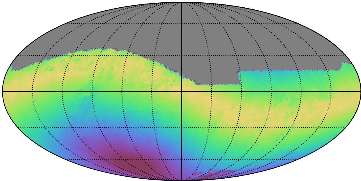
too_10_4v3.4_10yrs All sky i band: Max moonDistance
