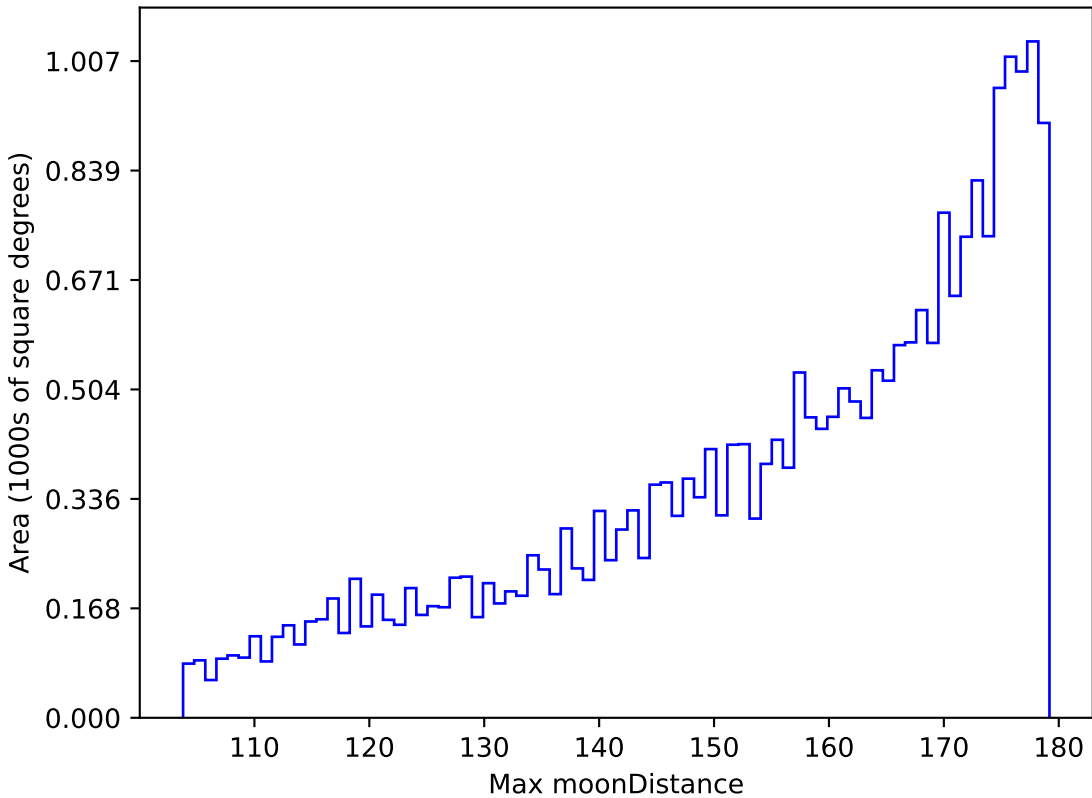
too_10_4v3.4_10yrs All sky i band: Max moonDistance
