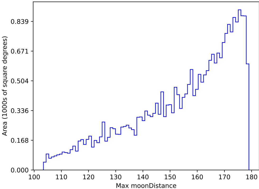
too_10_4v3.4_10yrs All sky g band: Max moonDistance
