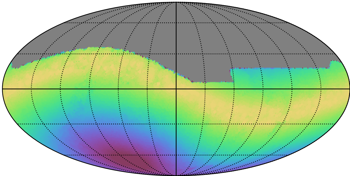
too_10_4v3.4_10yrs All sky all bands: Max moonDistance
