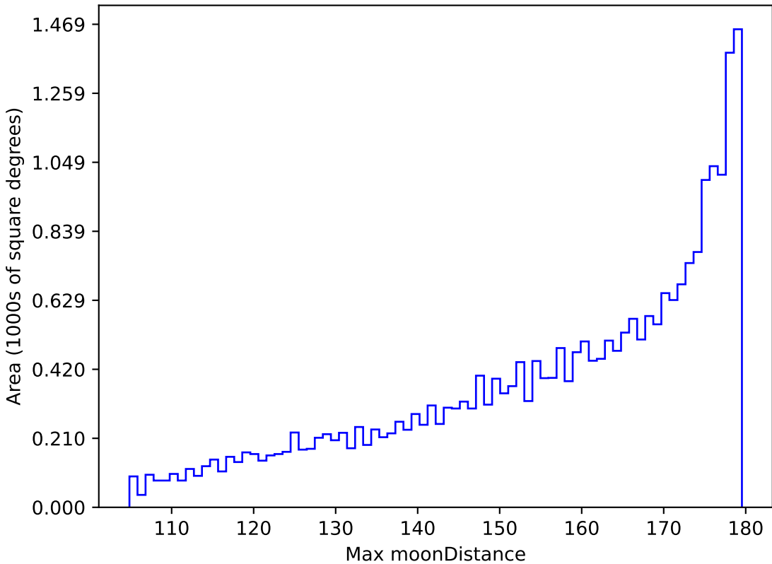
too_10_4v3.4_10yrs All sky all bands: Max moonDistance
