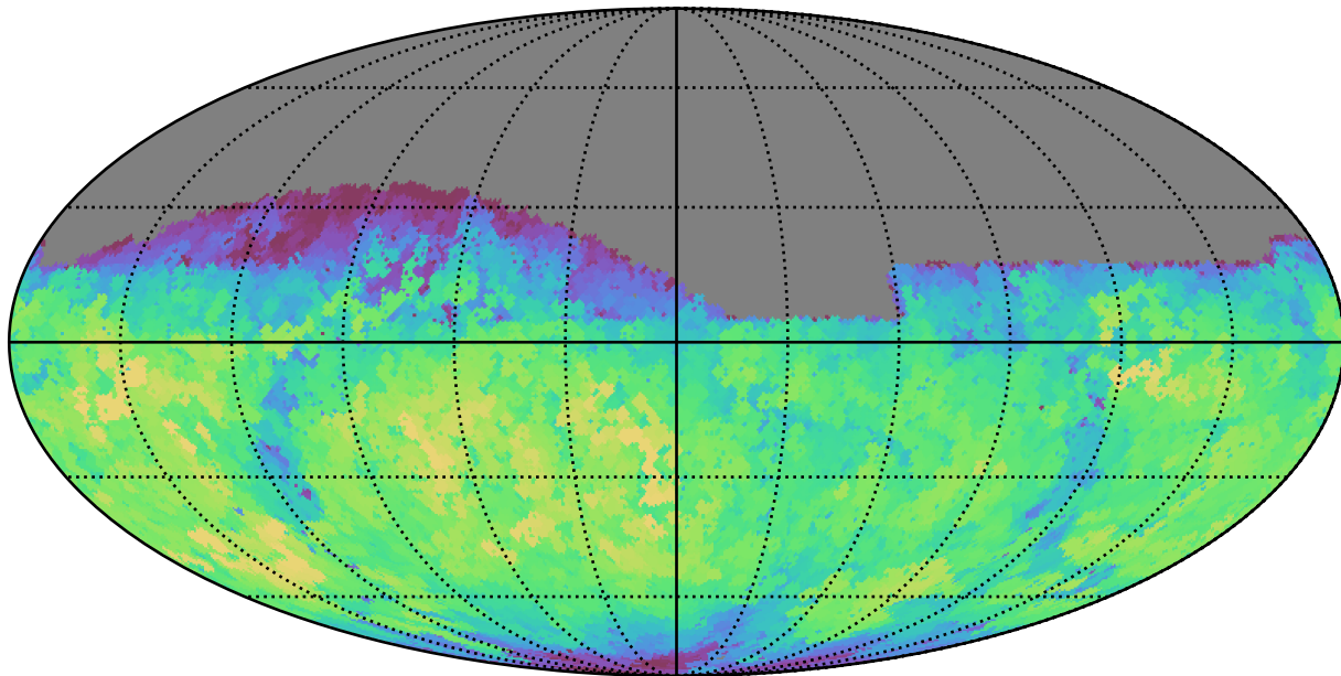
too_10_4v3.4_10yrs Yr 1 z band: Max fiveSigmaDepth
