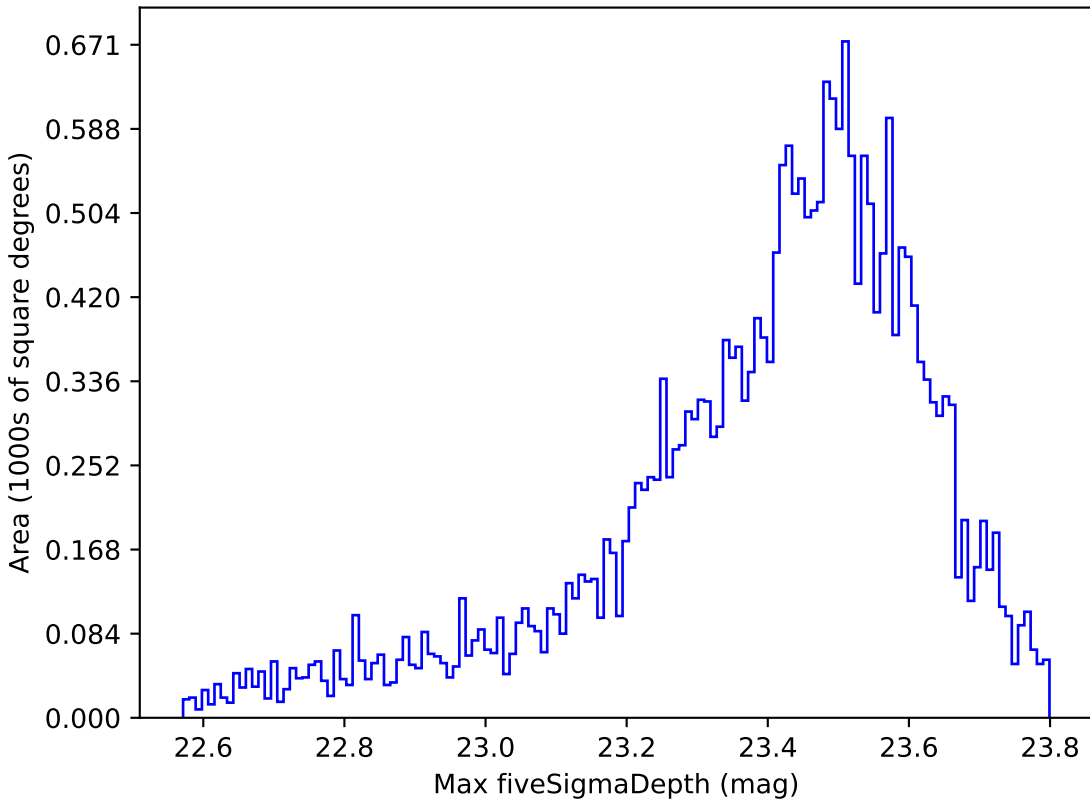
too_10_4v3.4_10yrs Yr 1 z band: Max fiveSigmaDepth
