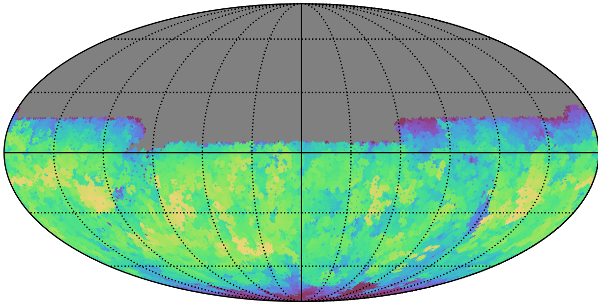
too_10_4v3.4_10yrs Yr 1 y band: Max fiveSigmaDepth
