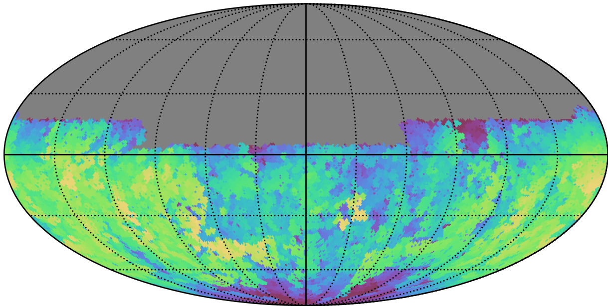
too_10_4v3.4_10yrs Yr 1 u band: Max fiveSigmaDepth
