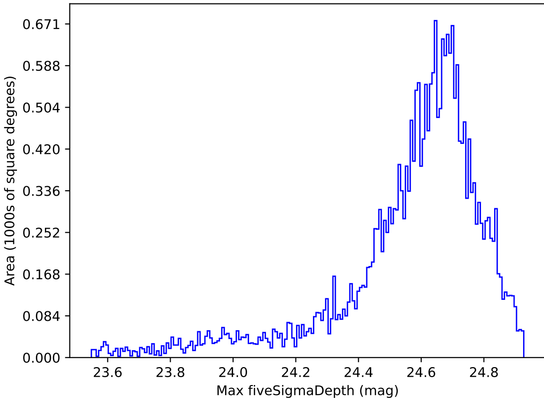
too_10_4v3.4_10yrs Yr 1 r band: Max fiveSigmaDepth
