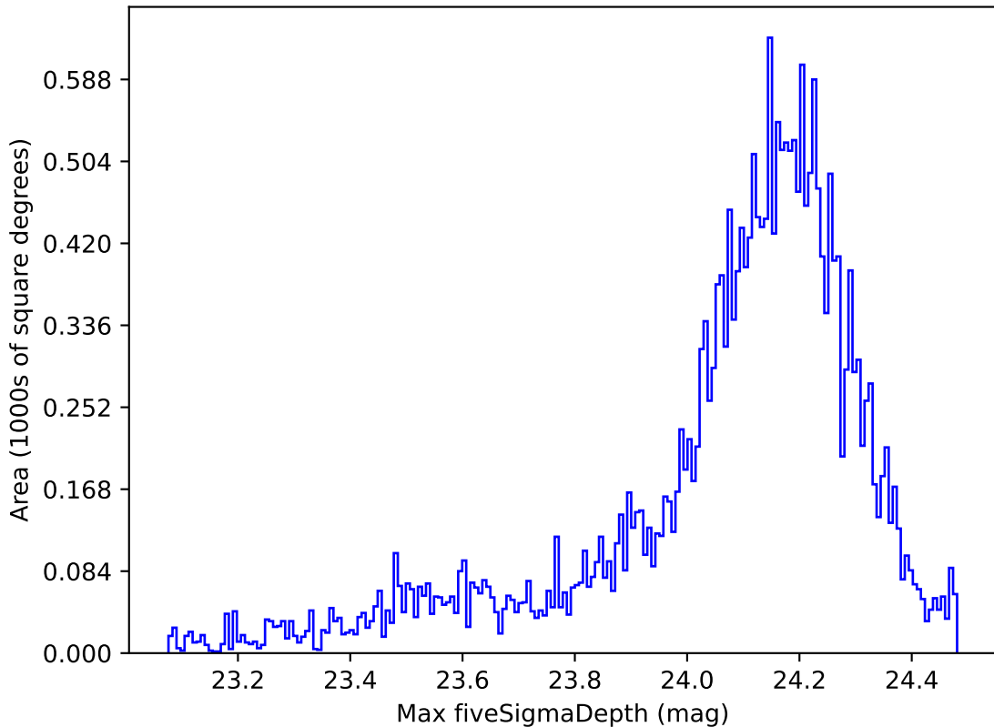
too_10_4v3.4_10yrs Yr 1 i band: Max fiveSigmaDepth
