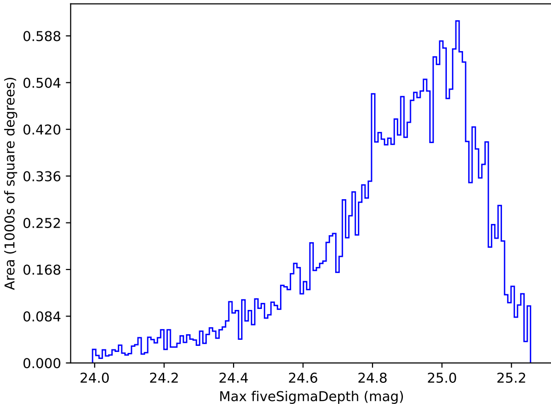
too_10_4v3.4_10yrs Yr 1 g band: Max fiveSigmaDepth
