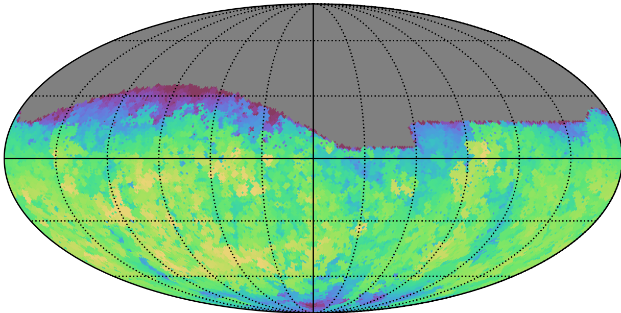
too_10_4v3.4_10yrs Yr 1 all bands: Max fiveSigmaDepth
