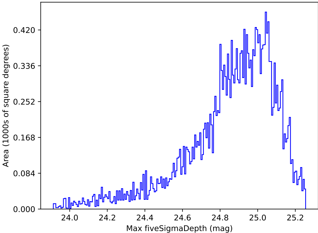
too_10_4v3.4_10yrs Yr 1 all bands: Max fiveSigmaDepth
