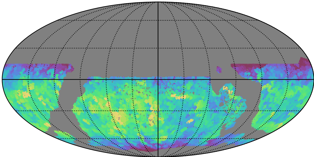
too_10_4v3.4_10yrs WFD z band: Max fiveSigmaDepth
