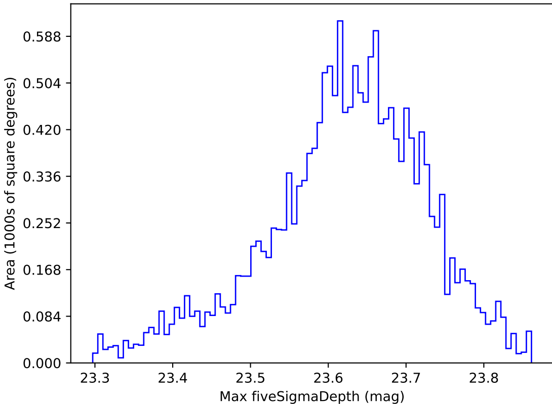
too_10_4v3.4_10yrs WFD z band: Max fiveSigmaDepth
