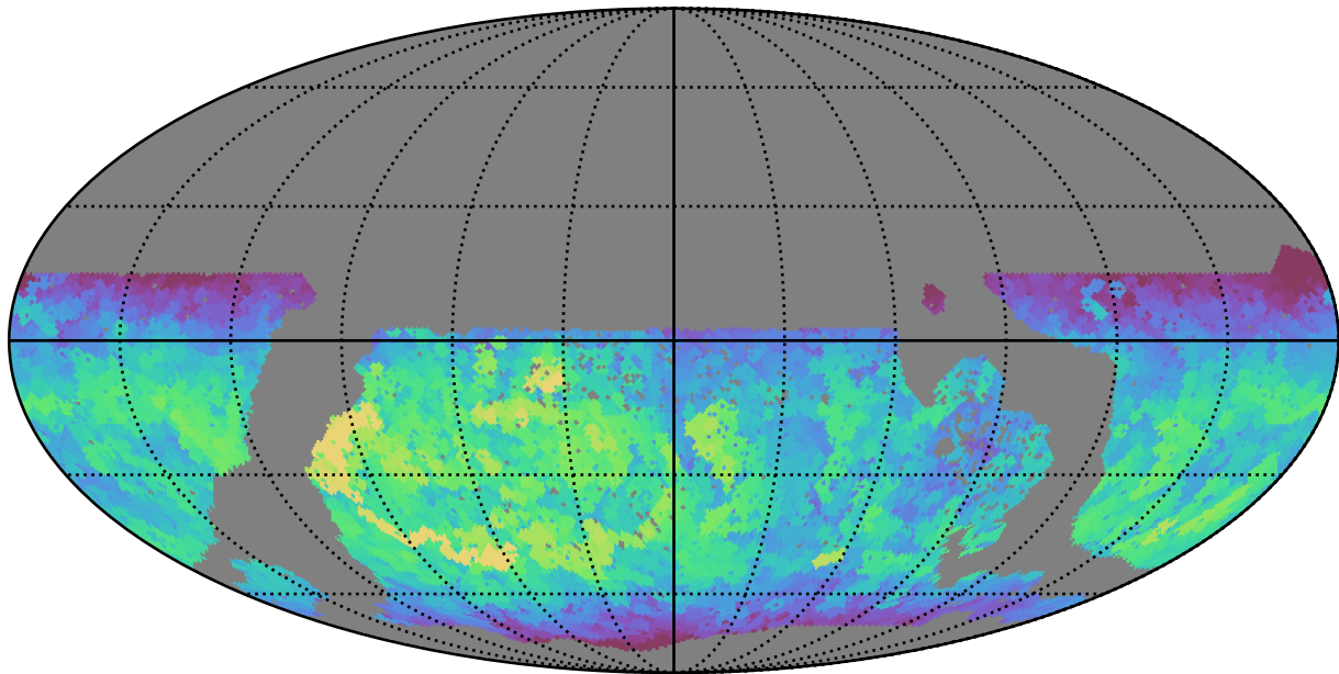
too_10_4v3.4_10yrs WFD y band: Max fiveSigmaDepth
