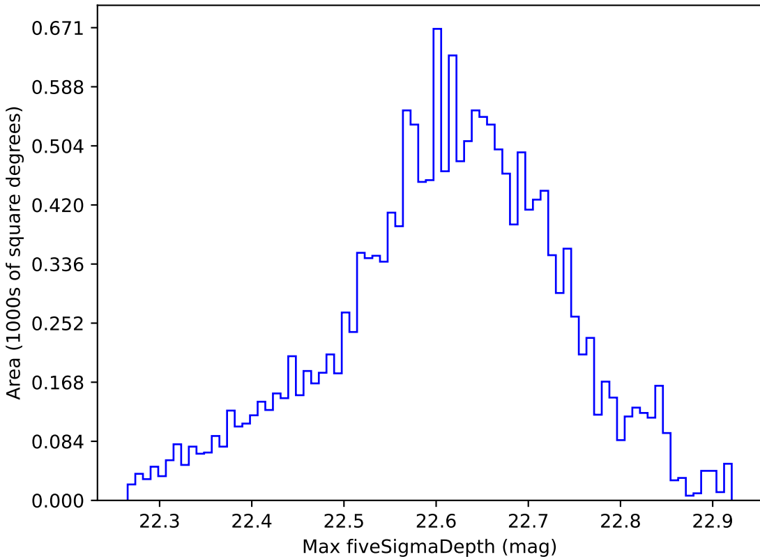
too_10_4v3.4_10yrs WFD y band: Max fiveSigmaDepth
